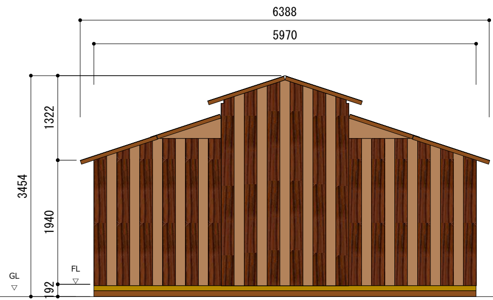
"A" elevation S = 1/60
