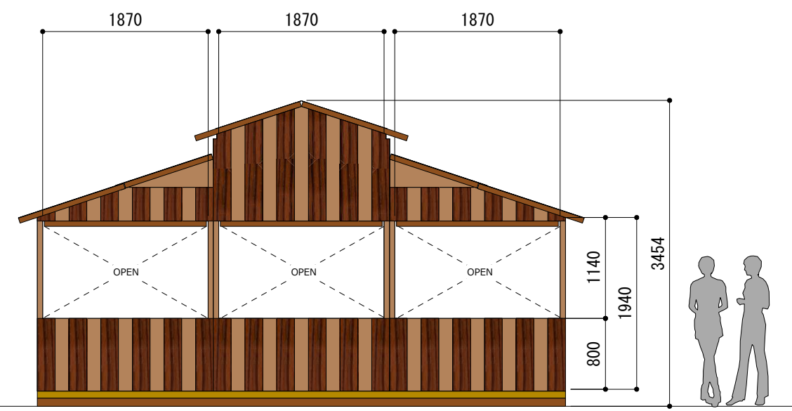
"C" elevation S = 1/60
