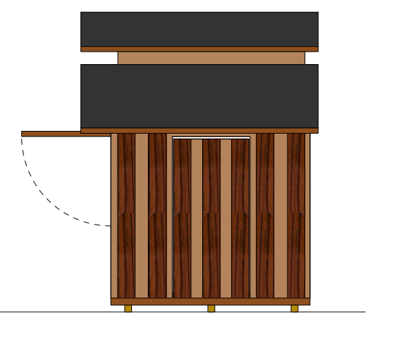
"D" elevation S = 1/60
