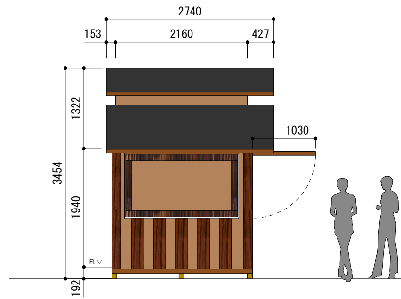
"B" elevation S = 1/60
